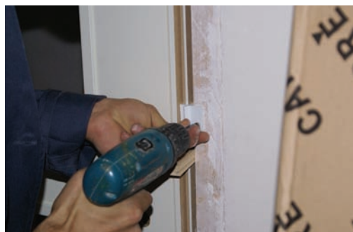
Fijar jambas. Fix the jambs. Fixer les jambes.
